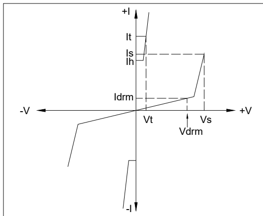
FIG1:V-I Characteristics
